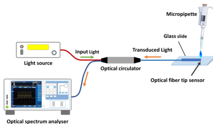
Figure 1. Experimental setup
