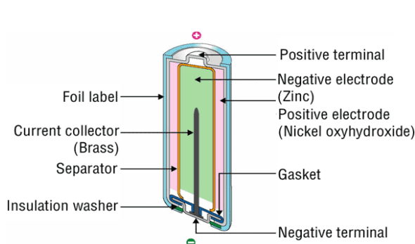
Figure 1. Schematic diagram of primary battery
