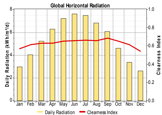
Figure 3. Monthly average daily radiation and clearness index
