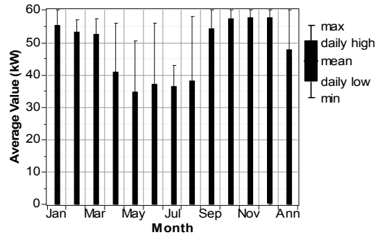
Figure 10. Monthly average output of fuel cell
