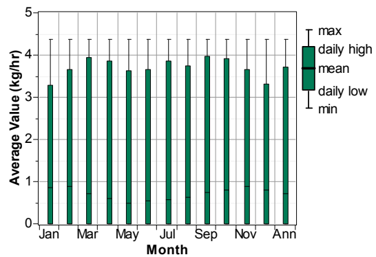
Figure 13. Monthly average output of the electrolyzer
