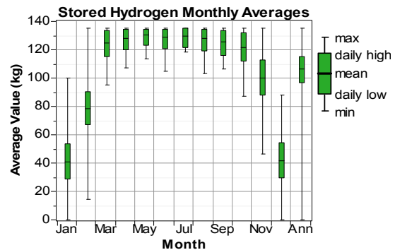
Figure 15. Monthly average stored hydrogen
