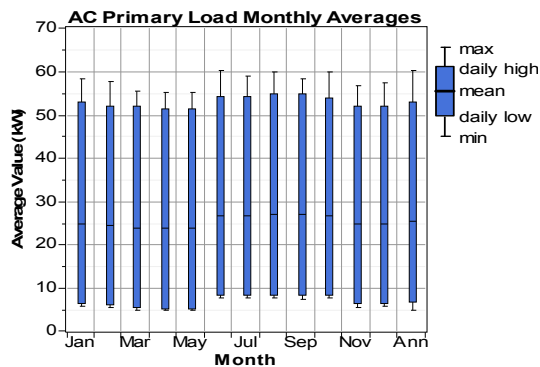
Figure 2. Monthly averages load profile
