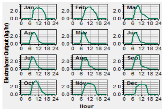
Figure 14. Daily profile of electrolyzer output
