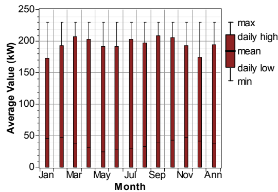
Figure 12. Monthly average electricity consumed by the electrolyzer
