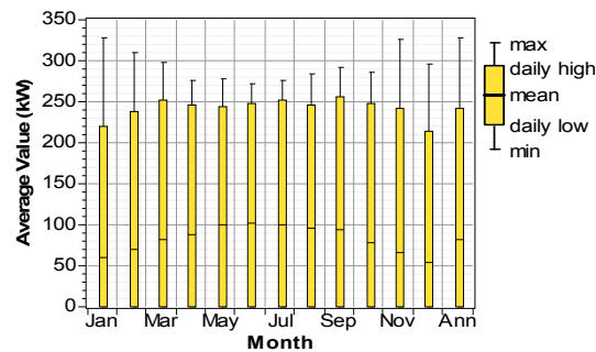
Figure 8. Monthly average output of PV
