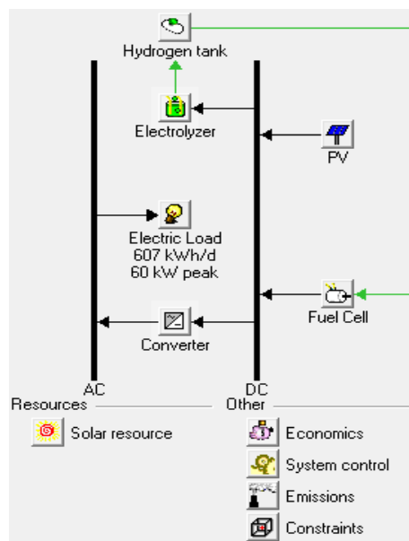
Figure 5. The configuration of a PV/FC hybrid power generation system in HOMER software
