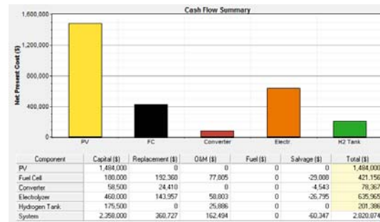
Figure 17. The cash-flow summary of the net present cost (25 years)
