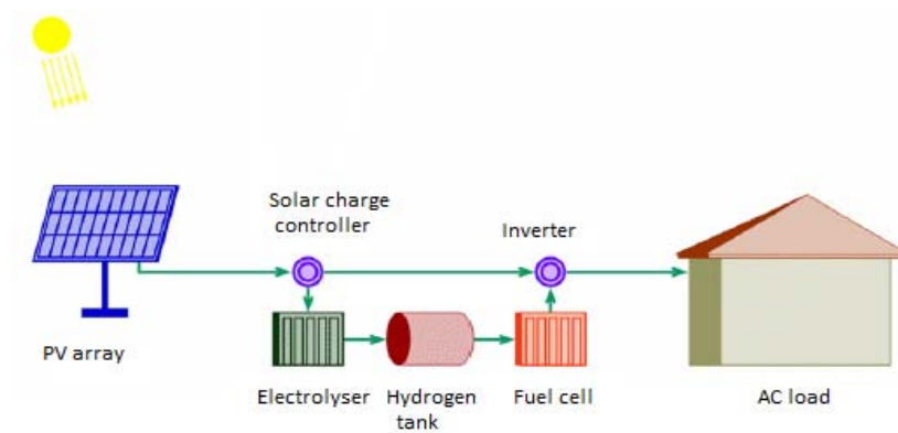
Figure 4. The configuration of a PV/FC hybrid power generation system
