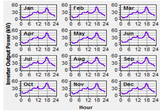
Figure 11. Daily profile of the inverter
