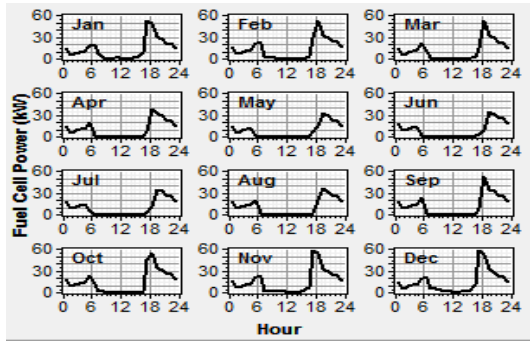
Figure 9. Daily profile of fuel cell out
