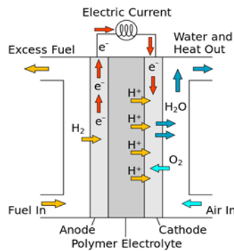
Figure 6. The basic principle of a fuel cell
