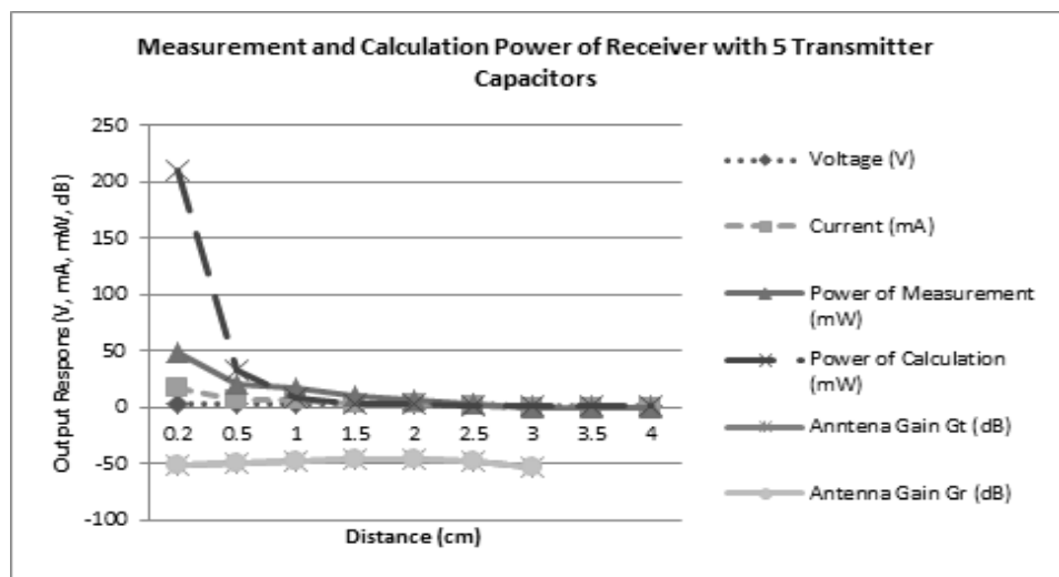
Figure 10. Chart of Measurement Result and Power Calculation, and Calculation of Transmitter Antenna Gain and Receiver Antenna Gain with 5 Capacitors of Transmitter
