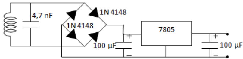
Figure 3. Receiver Circuit
