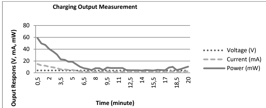
Figure 8. Test Result Chart of Voltage (V) Current (mA), Power (mW), Against Time (minute)
