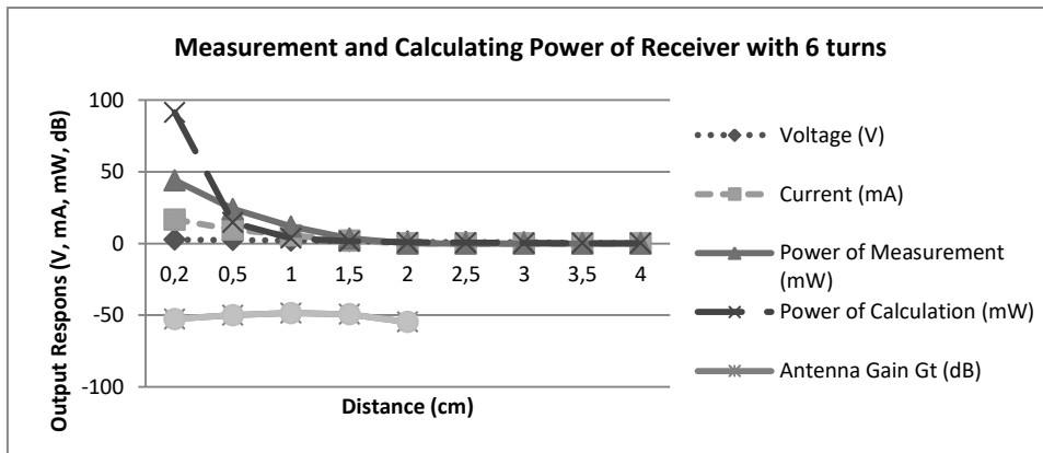
Figure 9. Chart of Measurement Result and Power Calculation, and Calculation of Transmitter Antenna Gain and Receiver Antenna Gain with 6 Turns of Antenna
