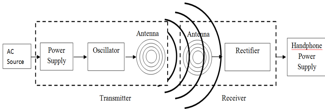
Figure 1. Block diagram of system design of the mobile phone wireless charger
