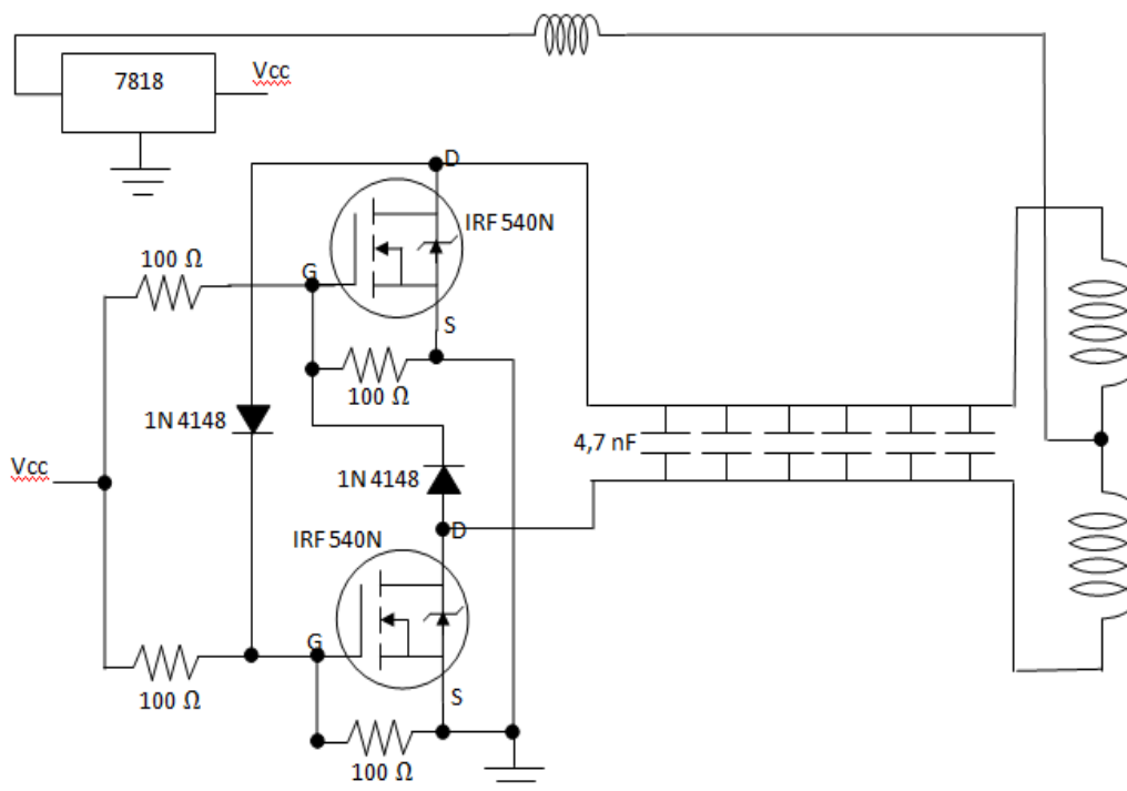
Figure 2. Oscillator Circuit
