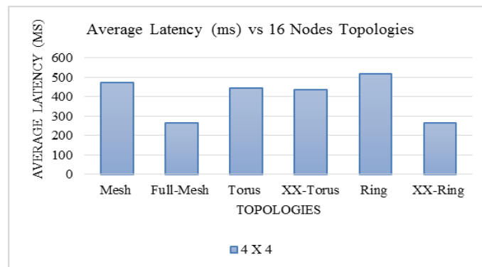
Figure 7. Average Latency (ms) of Different 16 Nodes Topologies
