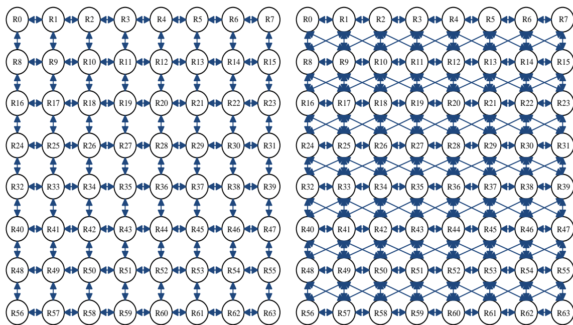
Figure 2. Mesh and Full-Mesh Topologies
