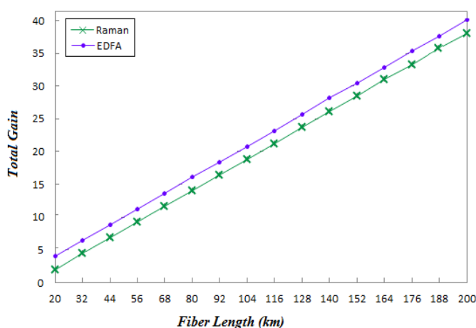
Figure 5. Total gain versus fiber length for the both optical amplifiers, Raman and EDFA
