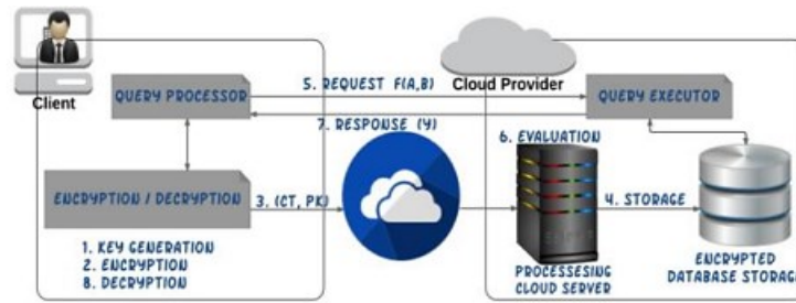
Figure 3. Applying homomorphic encryption to the cloud computing
