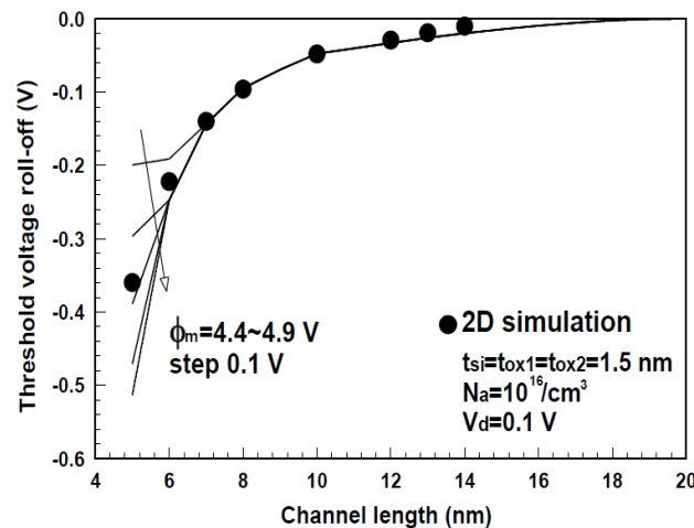
Figure 2. Threshold voltage roll-off of this model (solid line) and 2D Medici simulation (dot) under given conditions.
