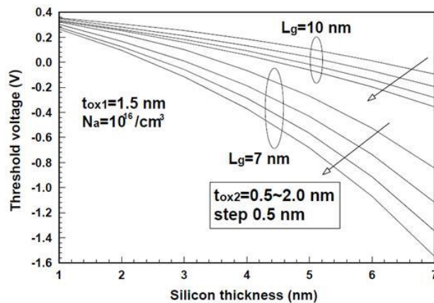
Figure 6. Threshold voltages for silicon thickness with a parameter of bottom gate oxide thickness.
