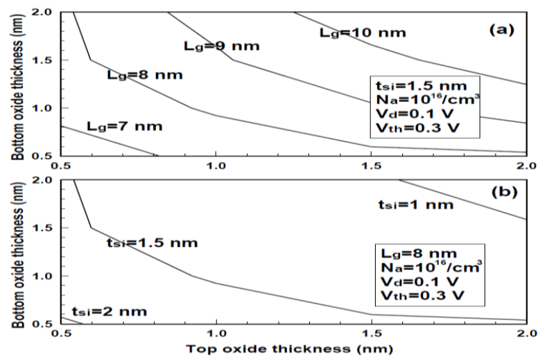
Figure 7. Contours for threshold voltage of 0.3 V for top and bottom gate oxide thickness in the case of (a) t_{si} = 1.5 nm and (b) L_g = 8 nm.
