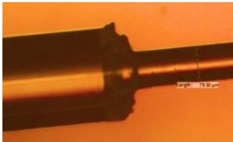
Figure 3. Etching process of fiber optic using HF 40% over 30 minutes
