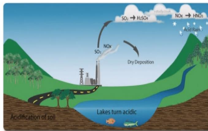
Figure 2. Acid rain scheme
