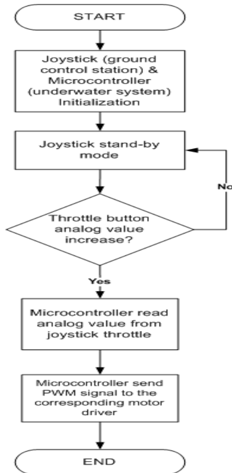
Figure 4. Thrust control system flowchart
