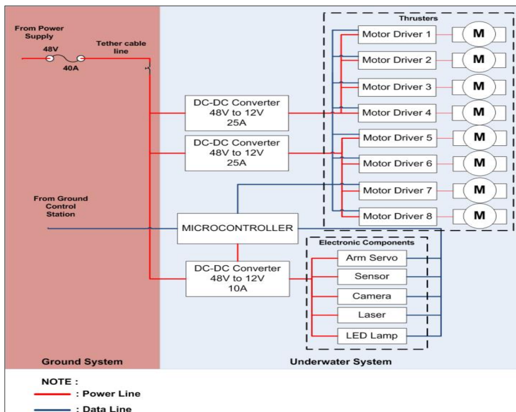
Figure 1. Proposed electrical power control system
