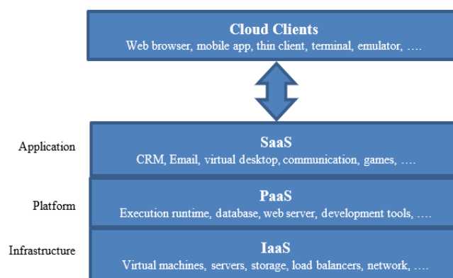
Figure 2. Different cloud service models
