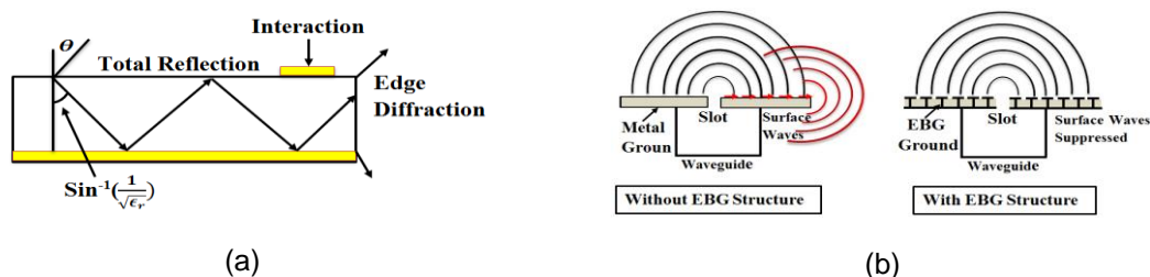
Figure 1. (a) Surface wave propagation in substrate of patch antenna, (b) propagation of surface waves using EBG structure
