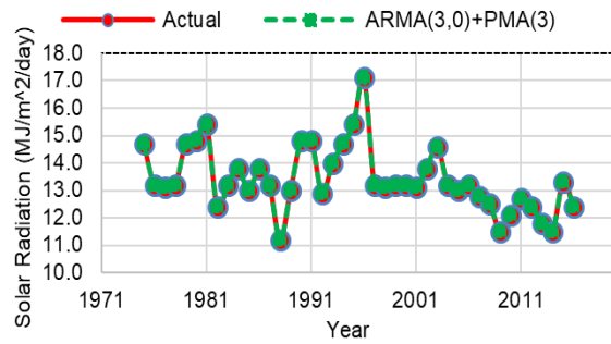
Figure 10. ARMA(3,0)+PMA(3) Forecasting
