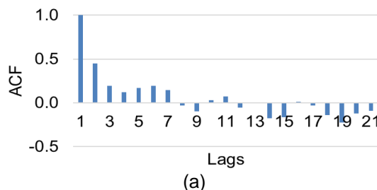
Figure 5. (a) Autocorrelation Function (ACF) of solar radiation (1971-2016) time series (b) Partial Autocorrelation Function (PACF) of solar radiation (1971-2016) time series
