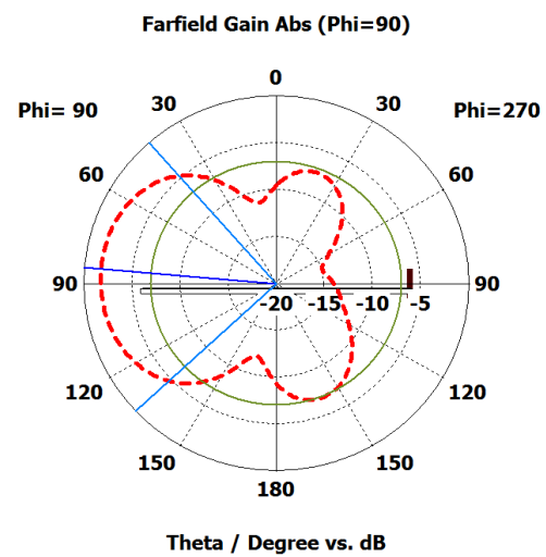
Figure 4. Radiation pattern for 2.8 GHz for monopole antenna
