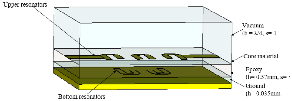
Figure 3. Multilayer construction of the proposed band-pass filter
