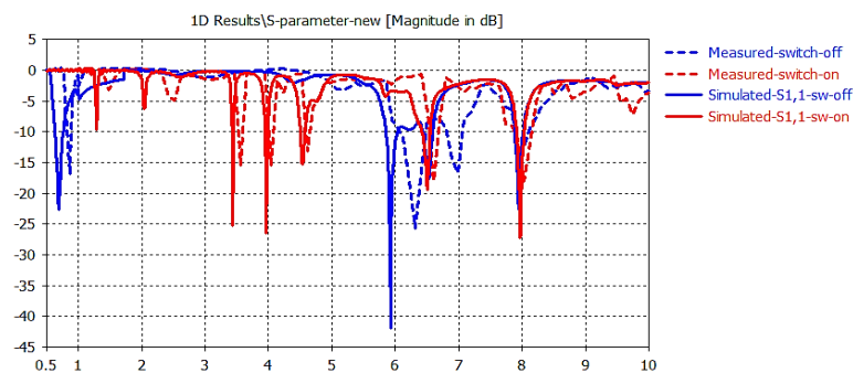
Figure 6. The simulated (S11) parameter versus frequency
