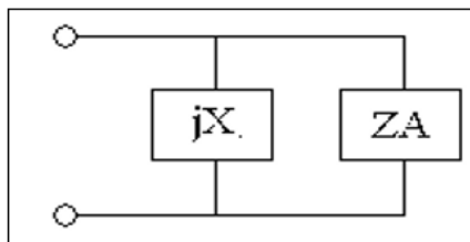
Figure 2. Equivalent circuit of PIFA antenna
