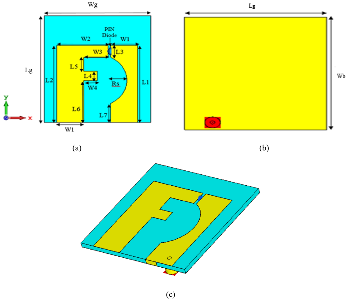
Figure 3. The proposed multiband reconfigurable PIFA antenna
