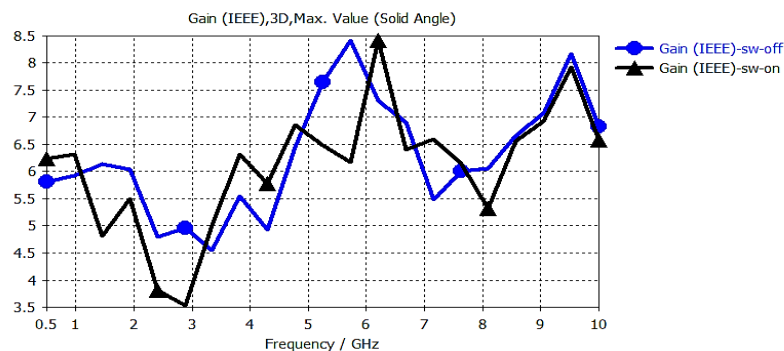
Figure 7. The gain variation with the frequency of the proposed reconfigurable PIFA antenna
