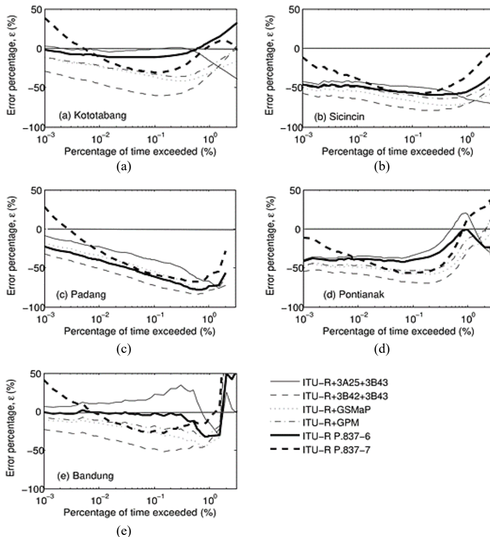
Figure 2. Percentage of errors between measurement and model results for each percentage of time exceeded
