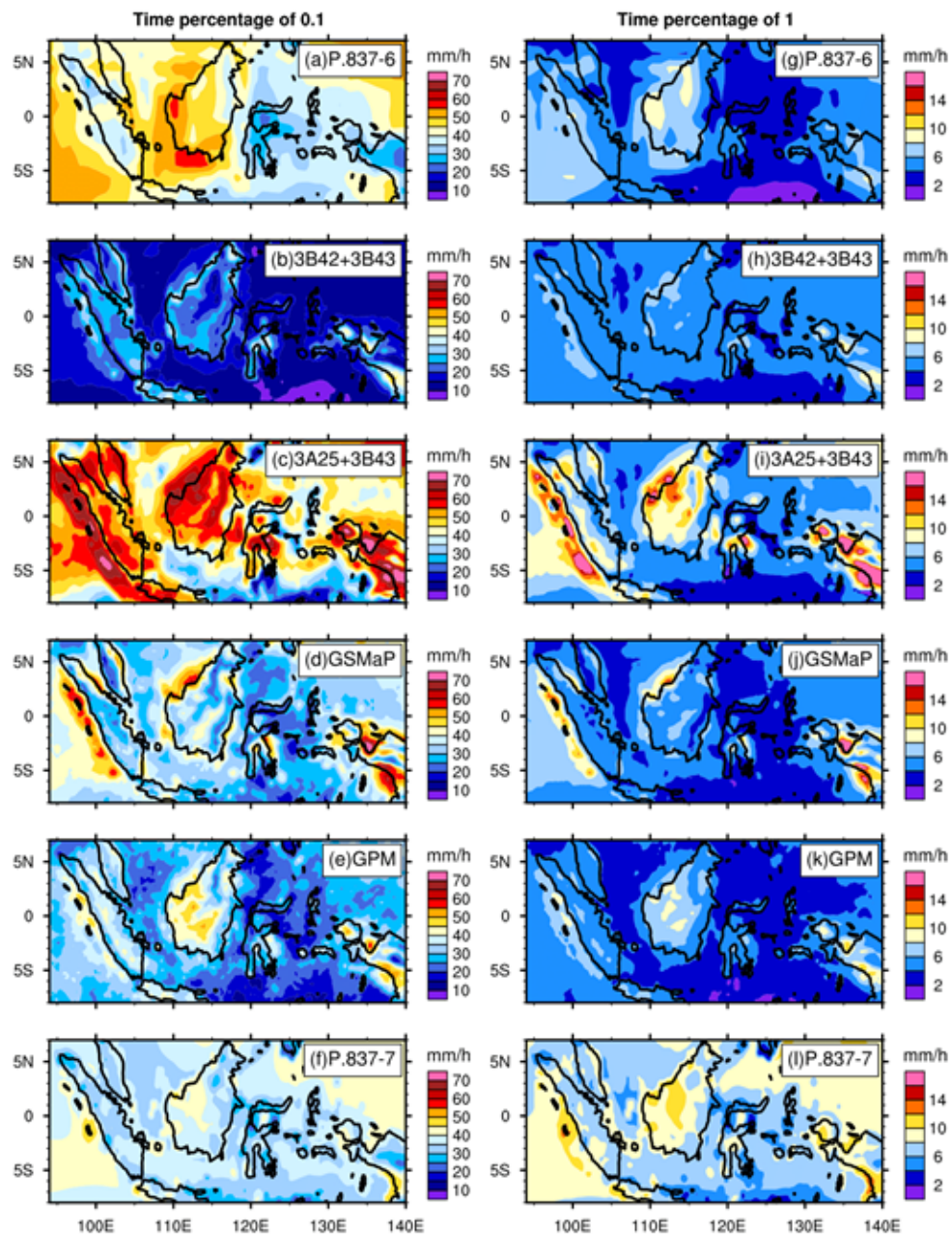
Figure 4. Distribution of rain rate for time percentage of 0.1% (left) and 1% (right) estimated by the default ITU-R P.837-6, modified ITU-R P.837-6, and ITU-R P.837-7
