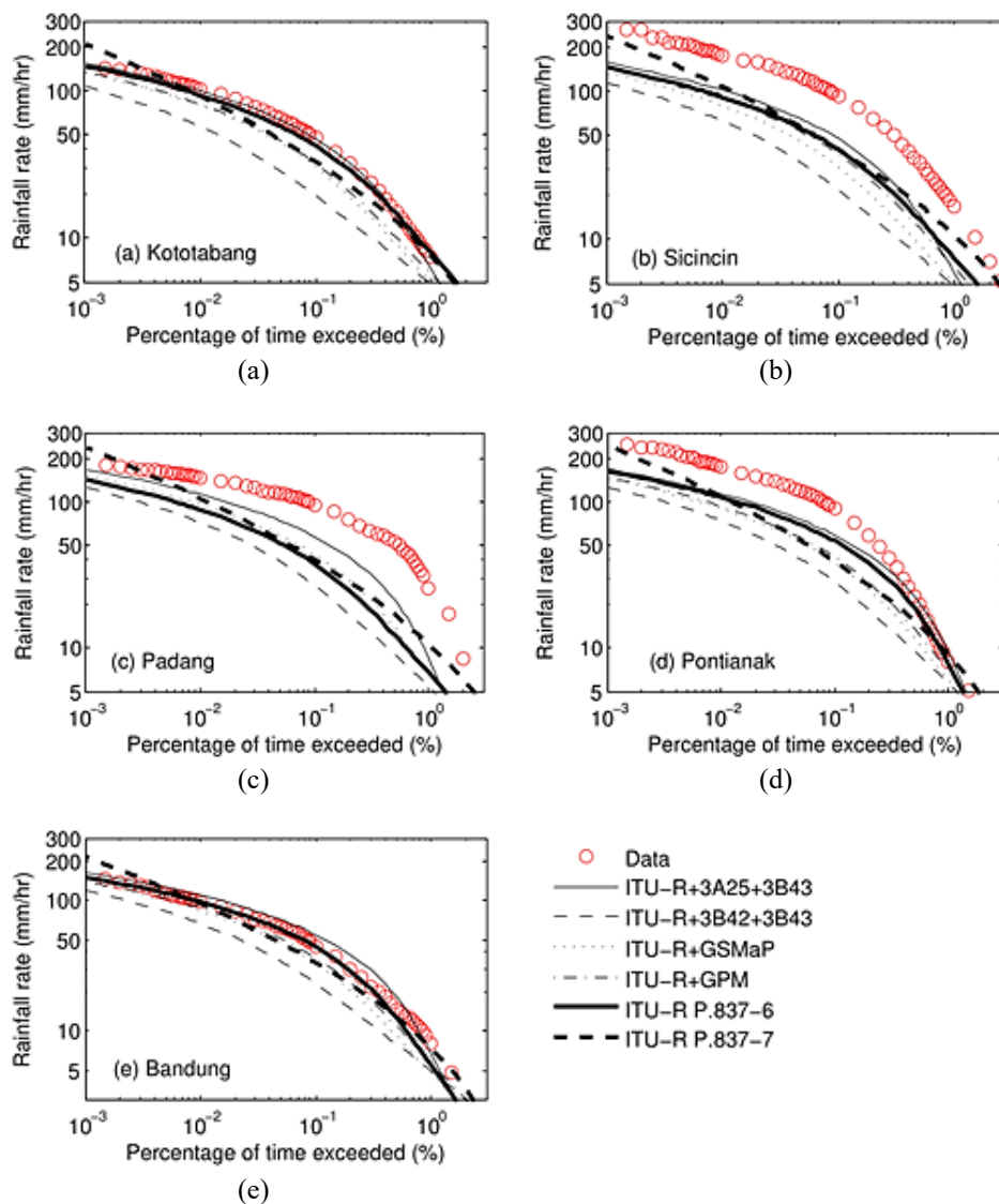
Figure 1. Comparison of cumulative distribution of rainfall rate from measurements and models
