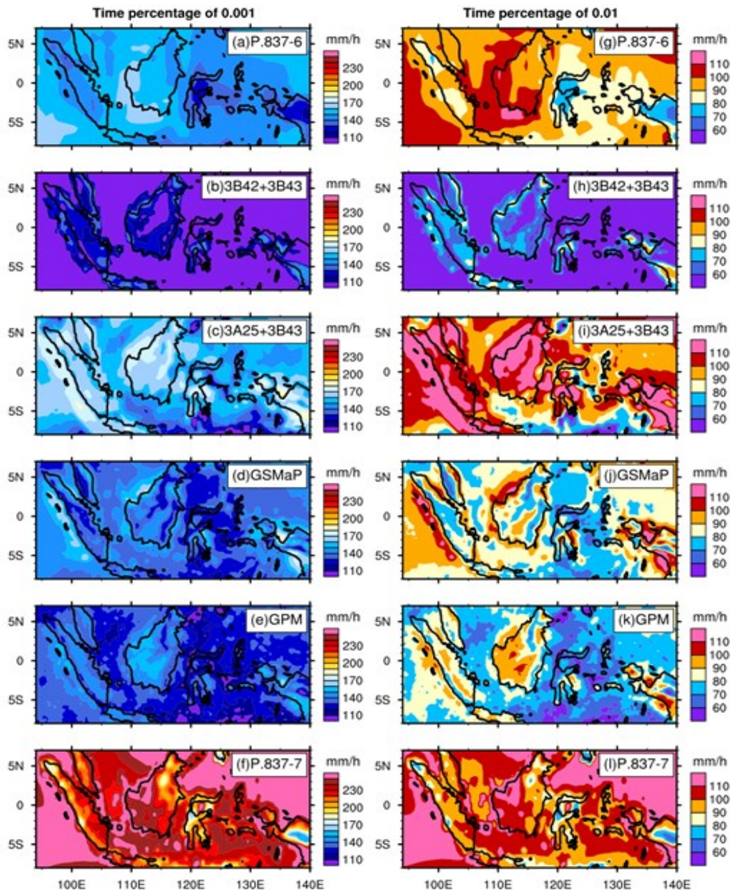
Figure 3. Distribution of rain rate for time percentage of 0.001% (left) and 0.01% (right) estimated by the default ITU-R P.837-6, modified ITU-R P.837-6, and ITU-R P.837-7
