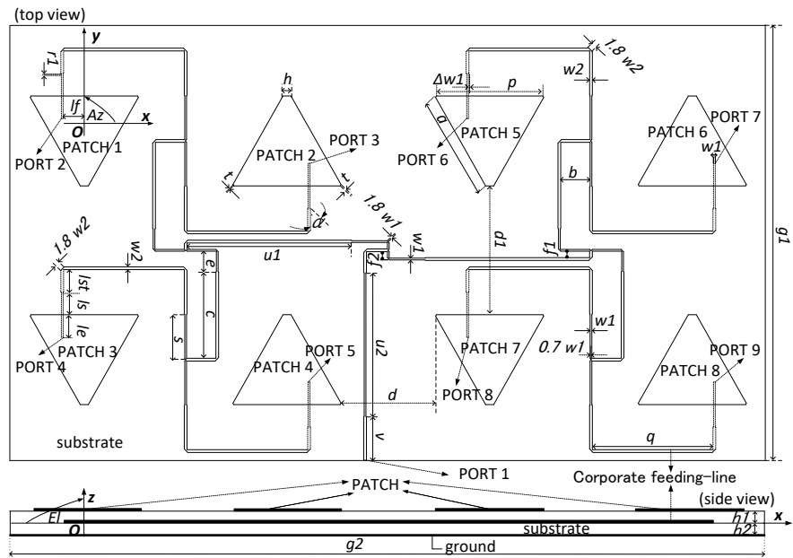
Figure 2. RHCP triangular array antenna 2x4
