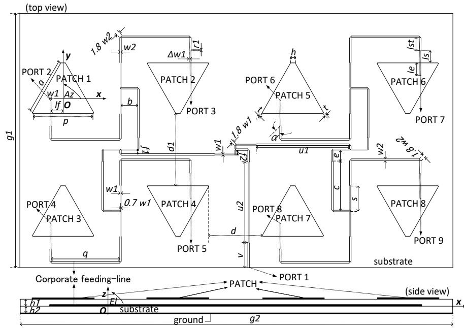
Figure 1. LHCP triangular array antenna 2x4
