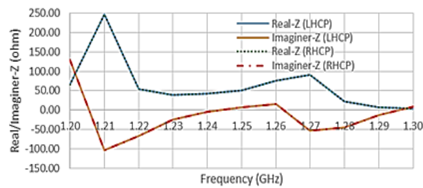
Figure 4. Input impedance, 2×4 patches
