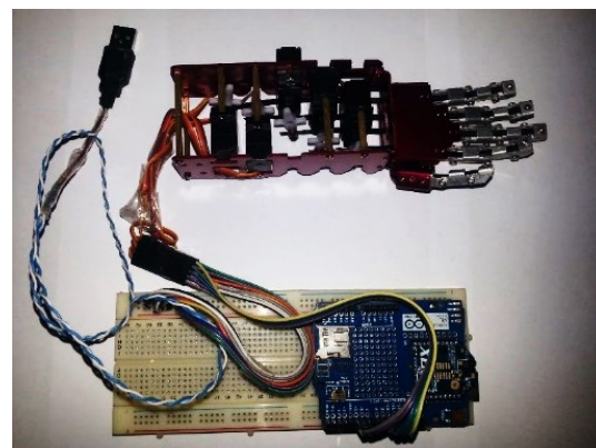
Figure 10. Robot side
