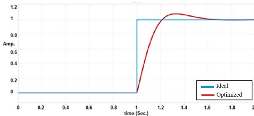
Figure 13. Step response of an optimized PID controller
