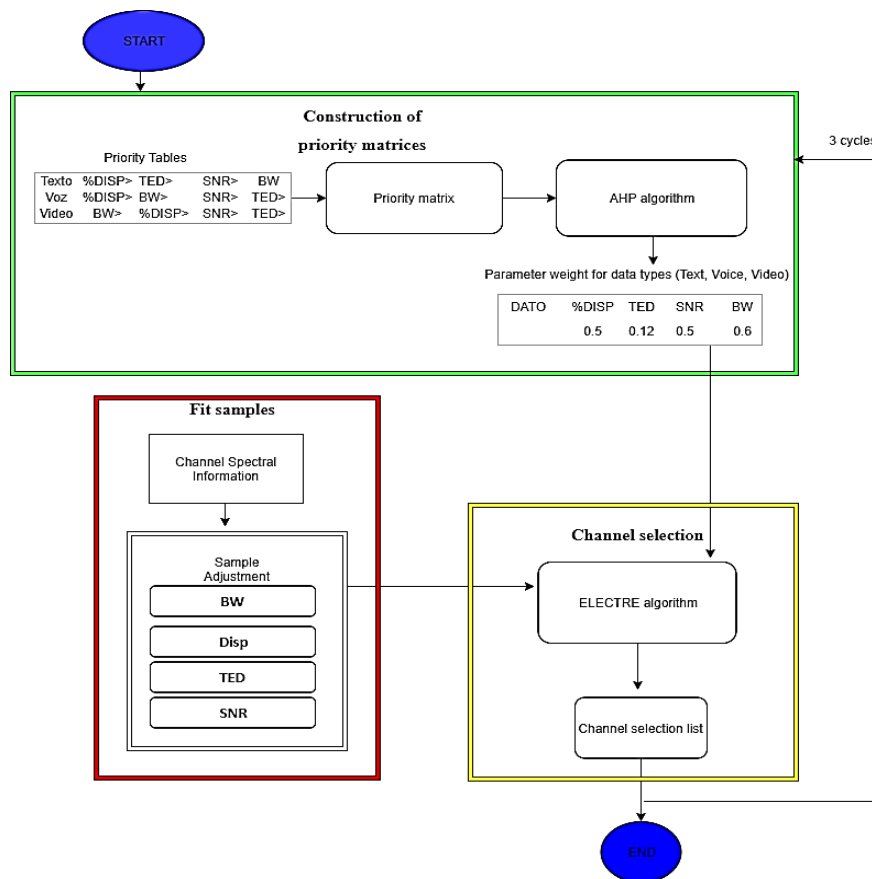
Figure 1. Proposed hybrid model
