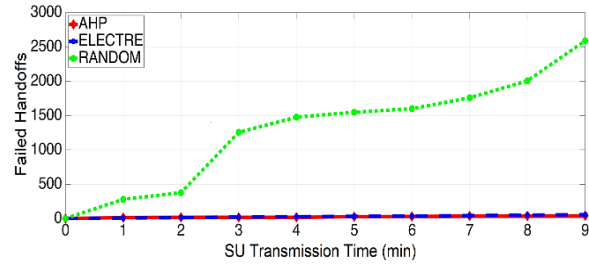
Figure 3. Failed handoffs
