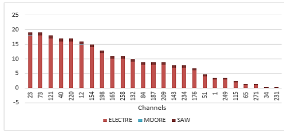
Figure 2. Unified results for the number of channels
