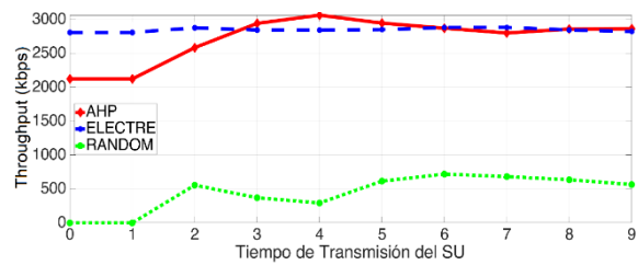
Figure 5. Throughput results for the analyzed algorithms
