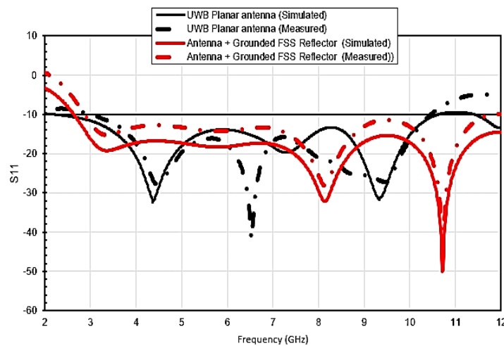
Figure 7. The simulated and measured magnitude of the reflection coefficient |S_{11}| for the suggested antenna in conjunction with the grounded reflector
