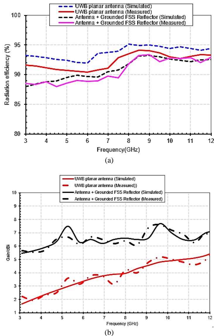
Figure 8. Predicted and measured outcomes (a) radiation efficiency (%) and (b) gain
