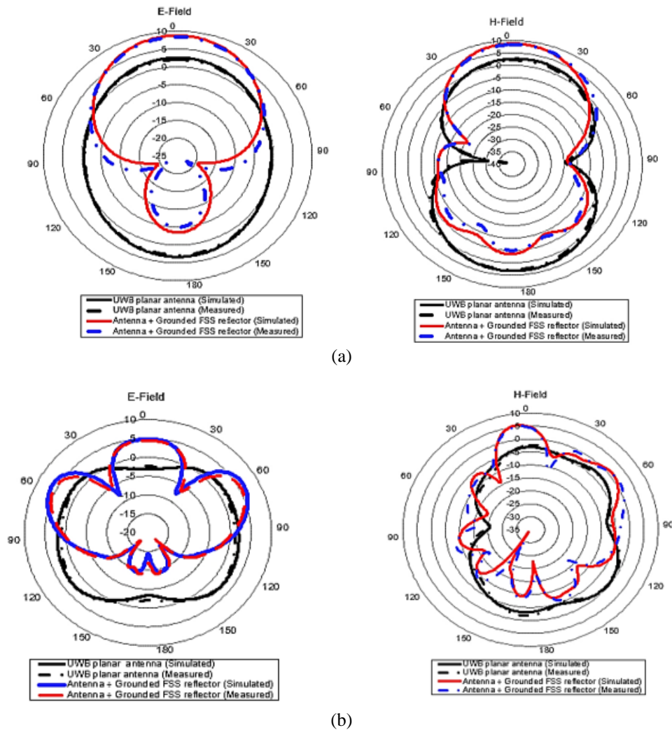
Figure 9. E and H field measurements of the proposed planar antenna with FSS grounded reflector at (a) 3 GHz and (b) 9 GHz
