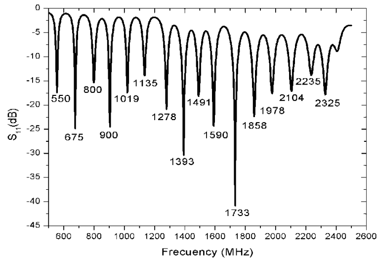
Figure 3. Results of simulation parameters S_{11} resonance frequencies
