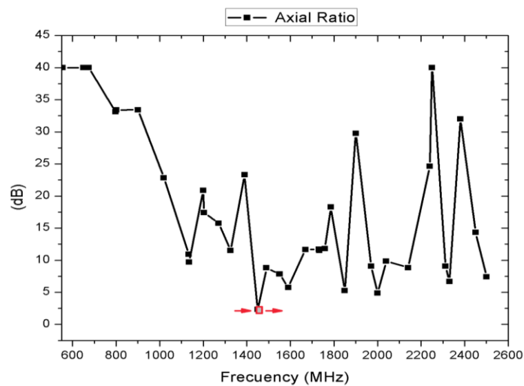
Figure 8. Axial ratio vs frequency simulated results
