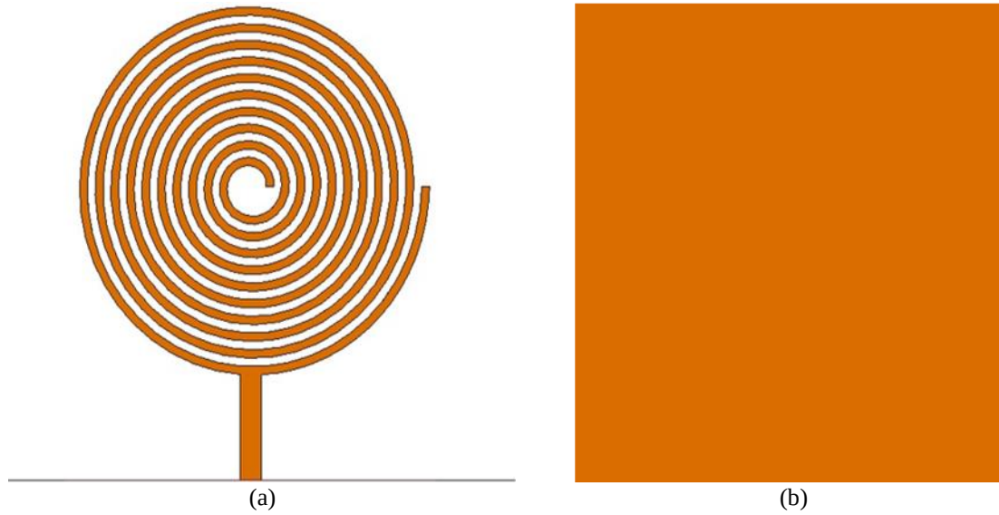
Figure 4. Initial design of the proposed single-turn antenna: (a) spiral radiating patch and (b) ground plane
