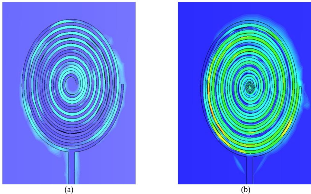
Figure 6. Simulation behavior of the surface current circulating through the windings: (a) less energy fluctuation and (b) greater coverage energy fluctuation
