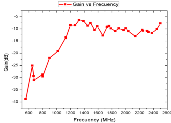
Figure 9. Gain vs frequency simulated results
