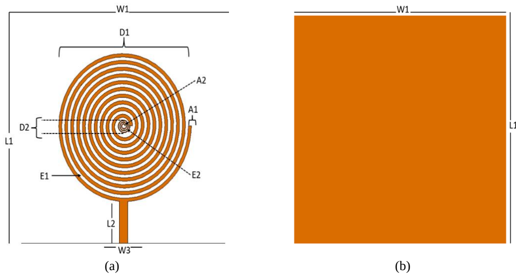
Figure 2. Design of the proposed antenna: (a) radiating patch with 10 turns, inner patch with 3 turns and (b) ground plane
