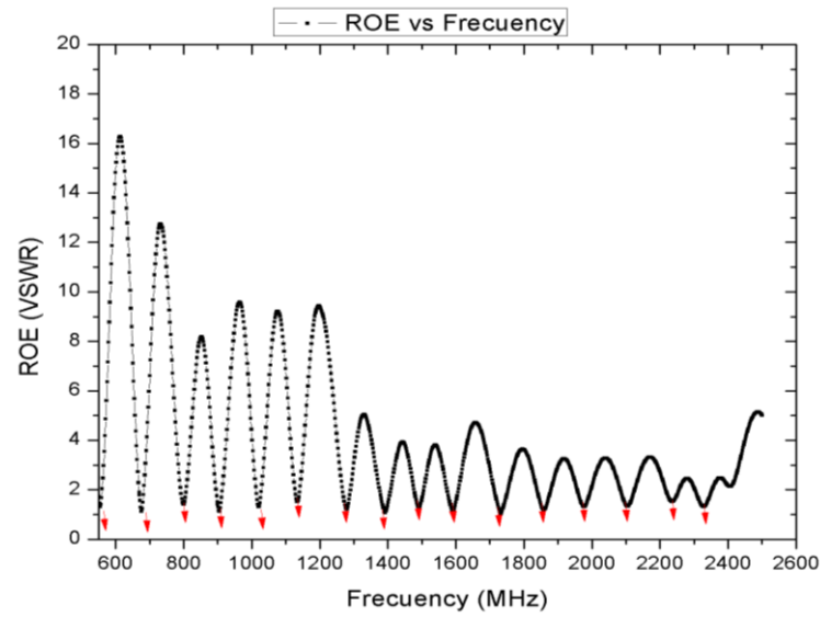
Figure 7. SWR simulated results. The red line represents the SWR value for each resonant frequency
