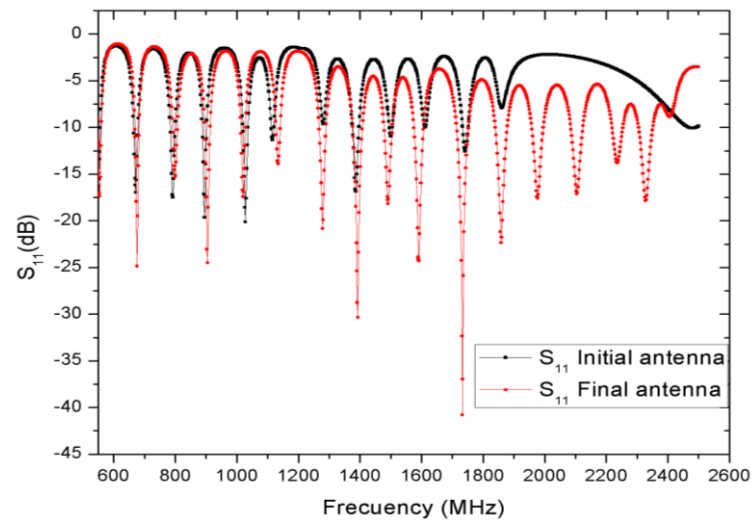
Figure 5. Parameter S_{11} frequency response of the simulation. Black line initial antenna, red line final antenna frequency respons
