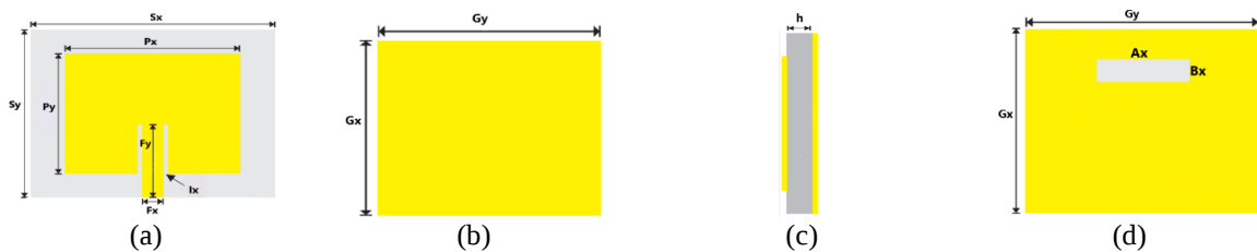
Figure 1. Conventional antenna and with antenna ground with DGS; (a) front view of conventional antenna, (b) back view of conventional antenna, (c) side view, and (d) ground after incorporating DGS
