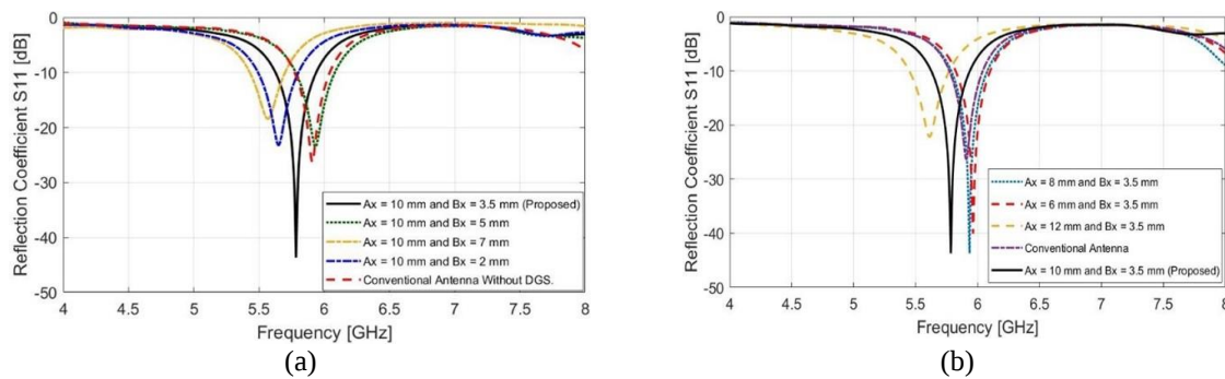
Figure 2. Parametric analysis of reflection coefficient; (a) corresponding to B_x when A_x is constant and (b) corresponding to A_x when B_x is constant
