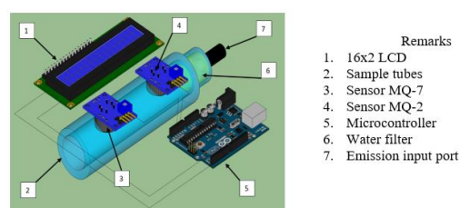
Figure 2. Device architecture
