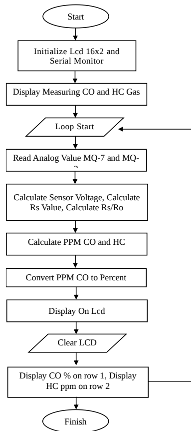
Figure 3. Software flowchart
