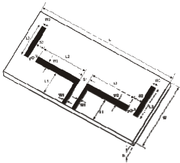
Figure 2. Fabricated antenna design
