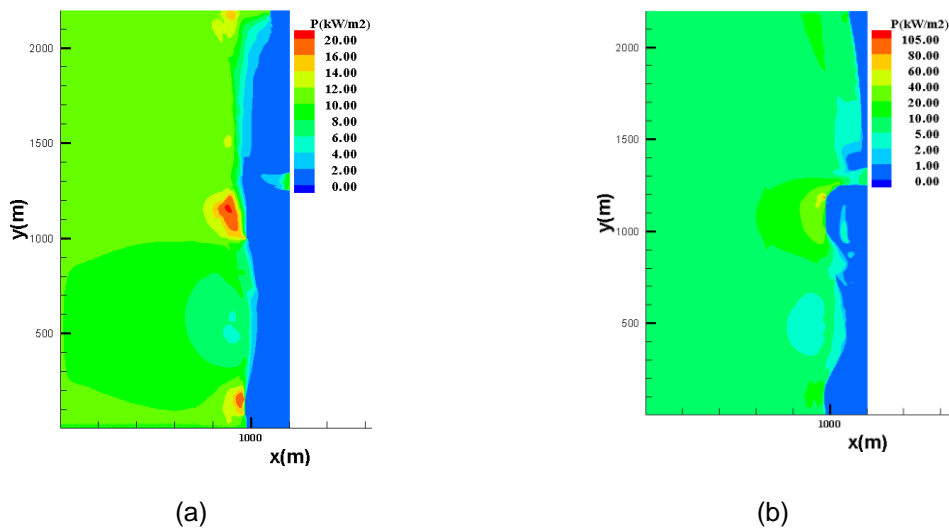
Figure 6. 2D-Simulated distributions of the power available when low tide currents (a) and high tide currents (b) in the Manado Bay
