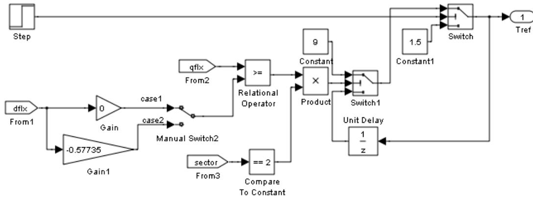
Figure 6. Generation reference torque from 1.5 to 9 Nm at a specific flux positions (i.e. case1 at the middle Sector II or case2 at the boundary Sector I and II).
