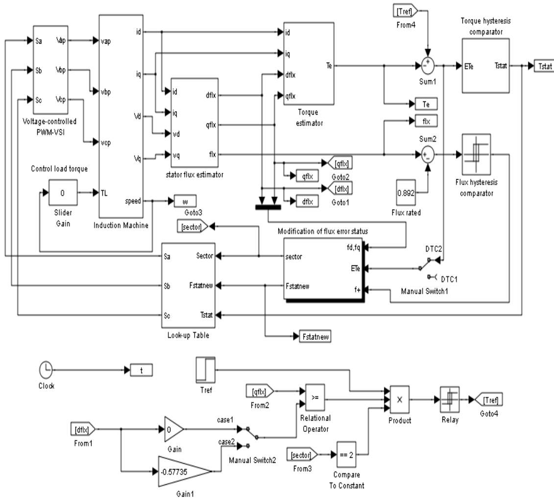
Figure 4. Simulink blocks of the DTC drive with the proposed block of modification of flux error status
