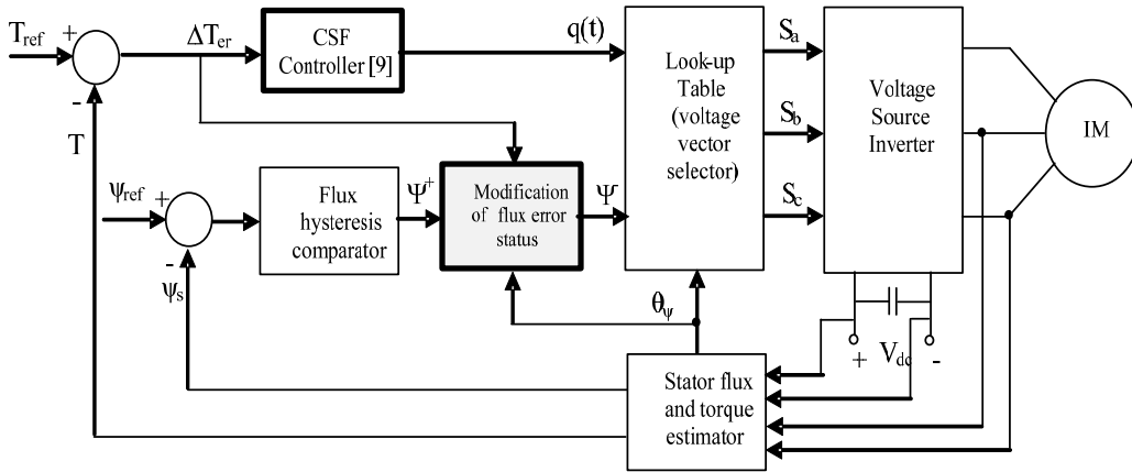
Figure 1. Proposed structure for dynamic overmodulation in DTC-CSF based
