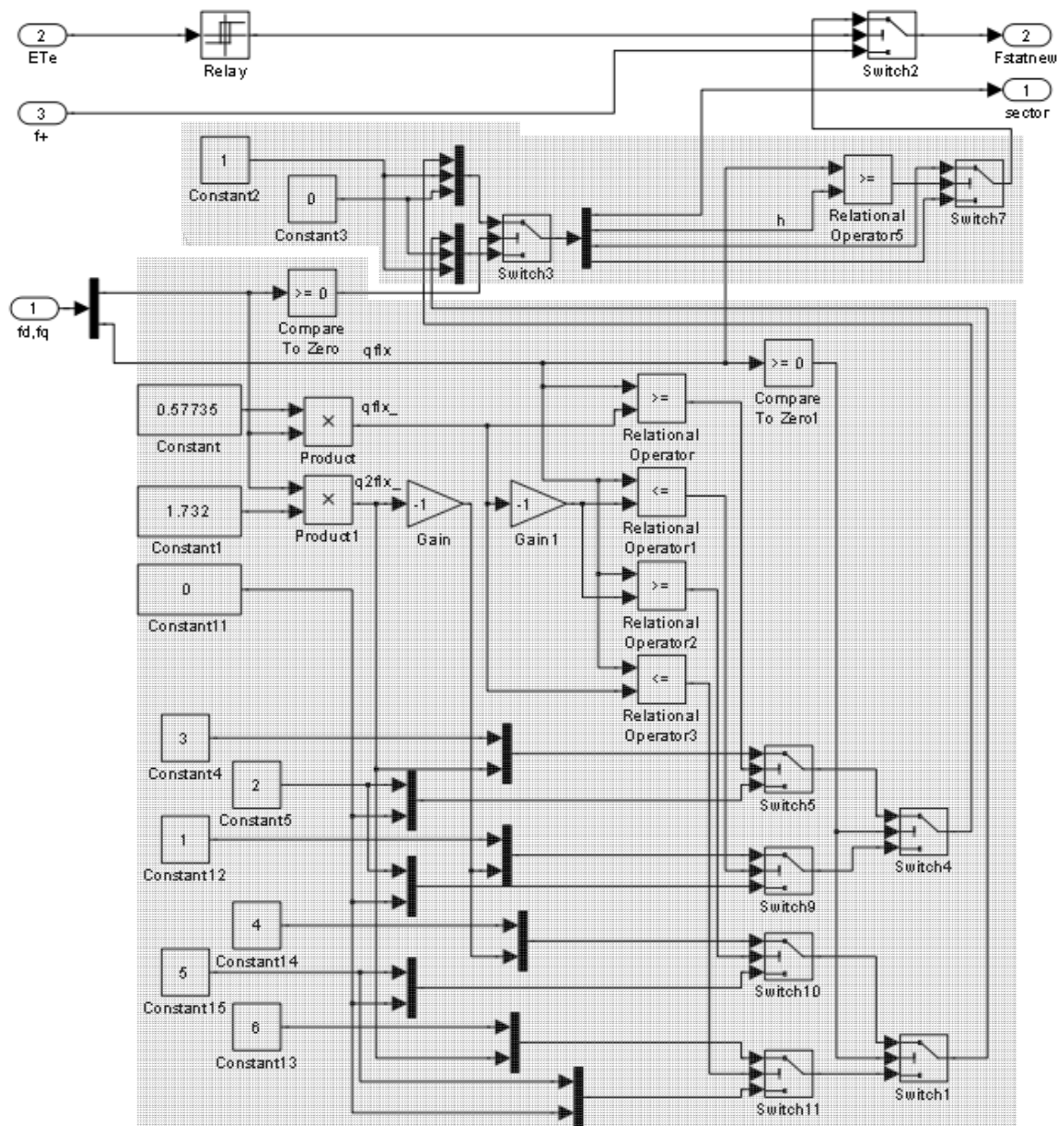
Figure 5. Identification of flux sector and determination of the appropriate flux error status in the block of modification of flux error status.
