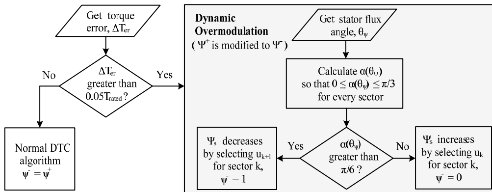
Figure 2. The operation of the proposed dynamic overmodulation
