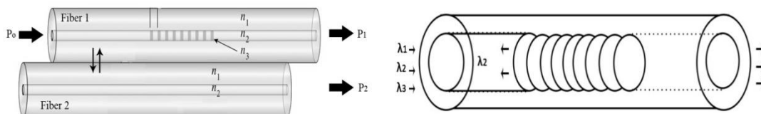
Figure 1. Power propagation of fiber; The leaf side is shown power propagation for input power P_o and output power P_1 and P_2 ; The right side is depicted schematic design of FBG [8]
