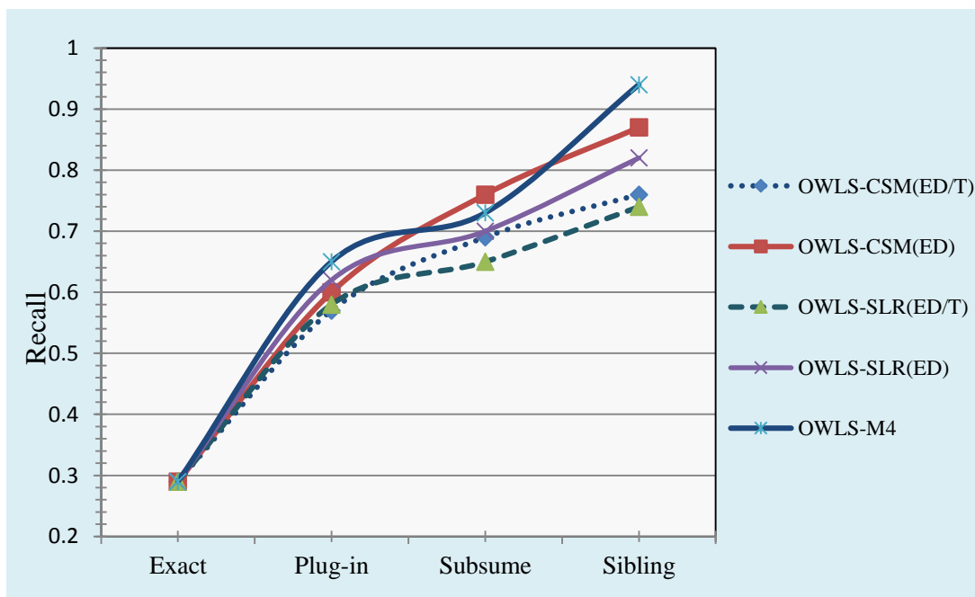
Figure 2. Recall
