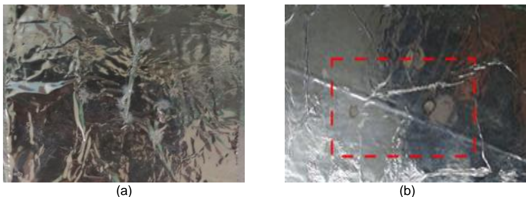
Figure 5. Direct effect of lightning strike: (a) The surface of 0.15mm aluminum foil with burning hole (b) The surface of 0.3mm aluminum foil without burning hole
