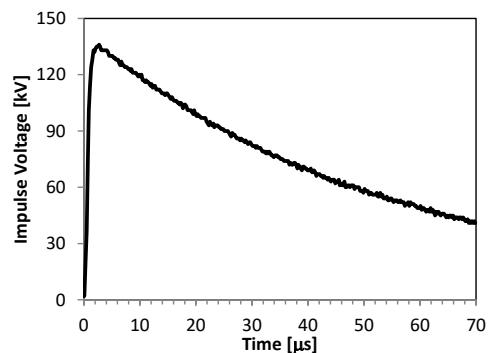
Figure 3. A standard impulse voltage 1.2/50μs which is supplied to high voltage electrode
