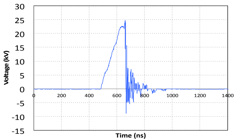
Figure 7. The output voltage of developed Blumlein line generator, the charging voltage is 9 KV.
