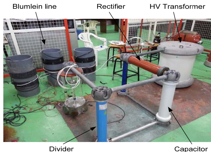
Figure 4. Photograph of the experimental arrangement to generate nanosecond pulses.
