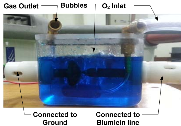
Figure 2. Hybrid discharge reactor
