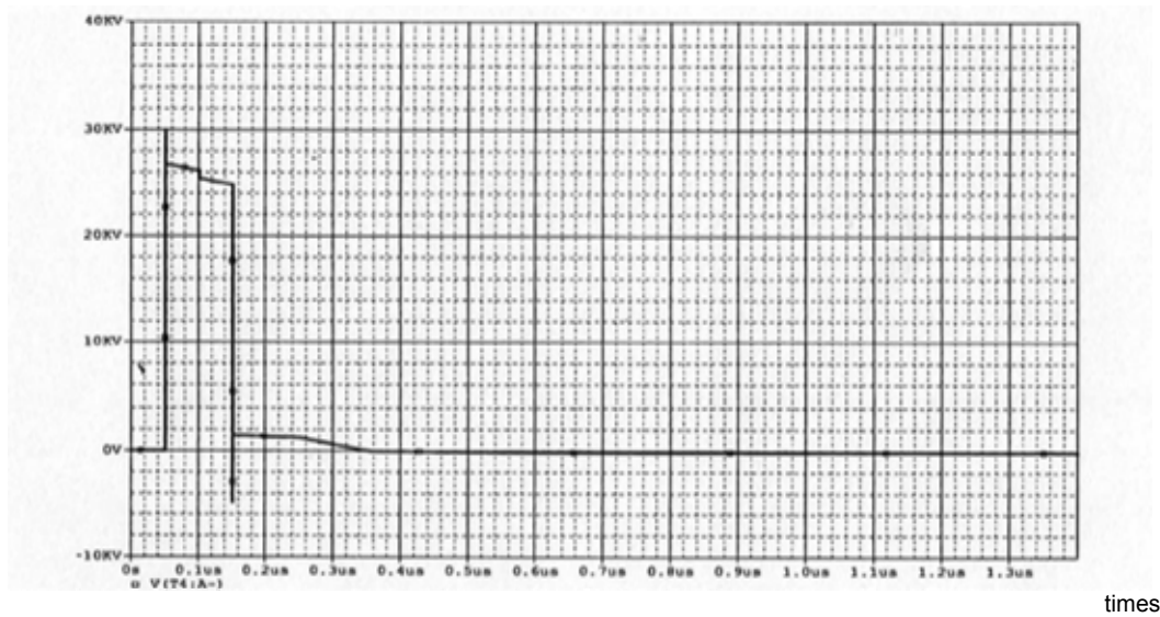
Figure 6. Simulation result of the Blumlein line.
