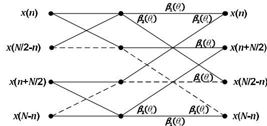
Figure 1. Butterfly of the ONMNT DIF algorithm, dotted and solid lines represent subtractions and additions respectively; \theta_1=k/2 is the rotation angle
